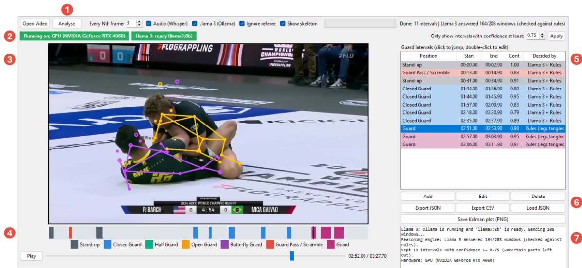
Figure 4.8: Grapple Eval desktop application after analysing the test video: (1) controls and progress, (2) hardware and Llama 3 status badges with the confidence filter, (3) video player with skeleton overlay, (4) colour-coded guard timeline, (5) interval table – clicking a row jumps the video to t_{start} , (6) editing and export buttons, (7) analysis log.
