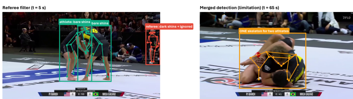
Figure 4.6: (a) Referee filter on the test video – the person with dark shins is ignored; (b) the main limitation – when the athletes are tightly entangled the pose model returns one skeleton for both bodies.
