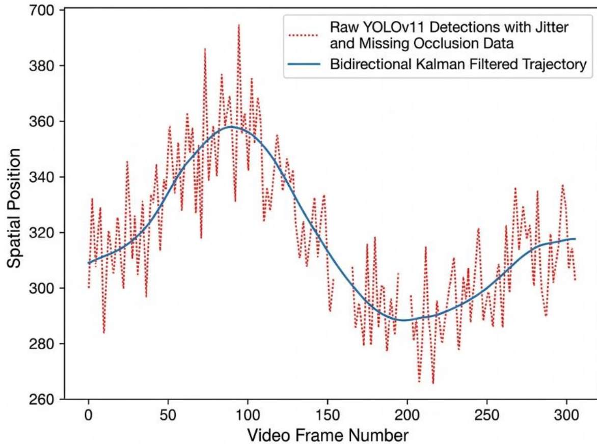
Figure 2.3: Raw YOLOv11 detections with jitter and missing occlusion data versus the bidirectional Kalman-filtered trajectory.
