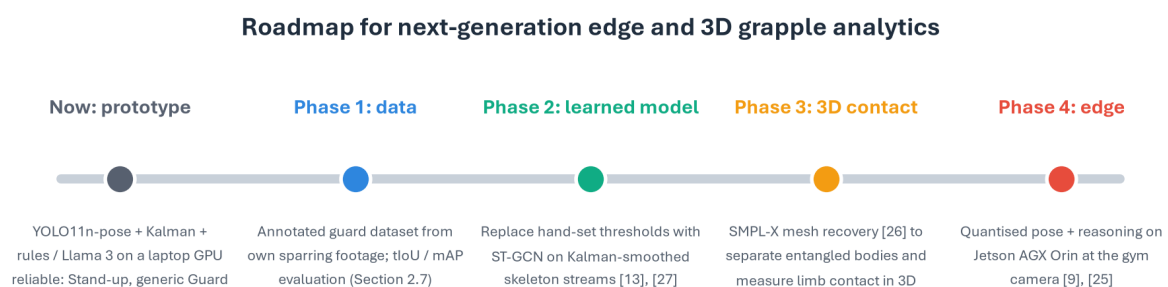
Figure 6.1: Roadmap for Next-Generation Edge and 3D Grapple Analytics.
